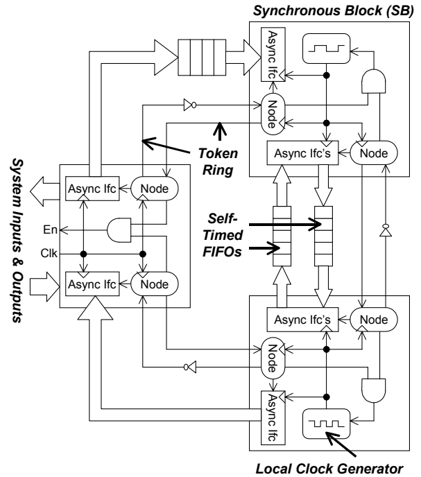
Figure 1. Synchro-tokens system architecture.
