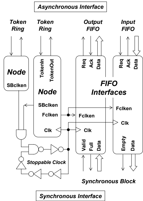
Figure 2. Wrapper logic: Nodes, FIFO interfaces, and a stoppable clock.
